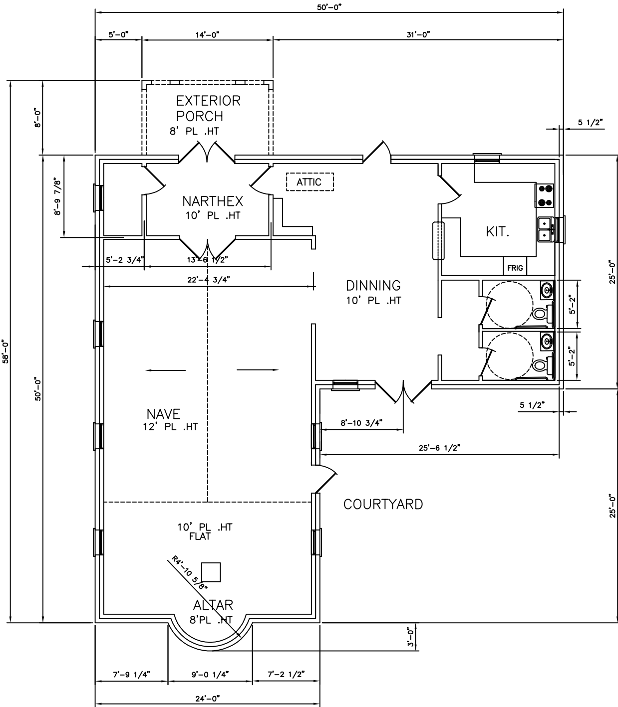
FLOOR PLAN-2 WITH DIMENSIONS
