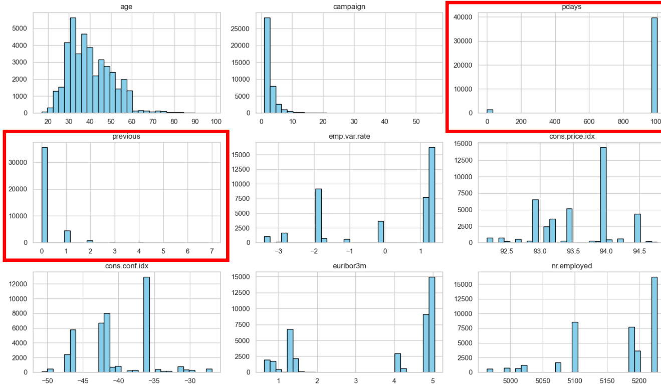
Histograms of Numerical Variables (Raw Data)
