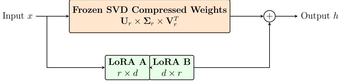
Figure 4: Our Proposed SVD-LoRA Architecture. The original base weights are entirely discarded and replaced by their frozen truncated SVD approximation. Trainable LoRA adapters operate in parallel to the compressed SVD path to recover the lost semantic fidelity.
