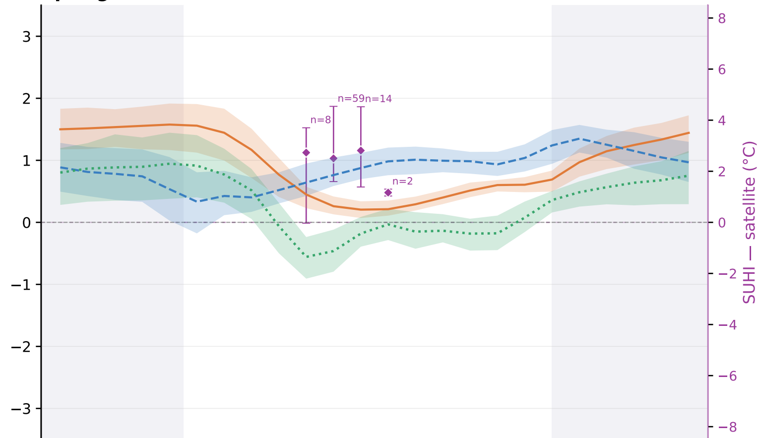
Spring (MAM)
