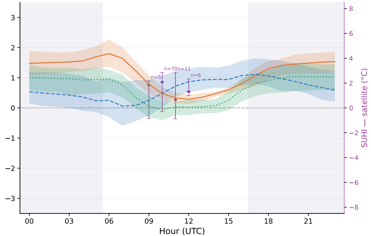
Autumn (SON)
