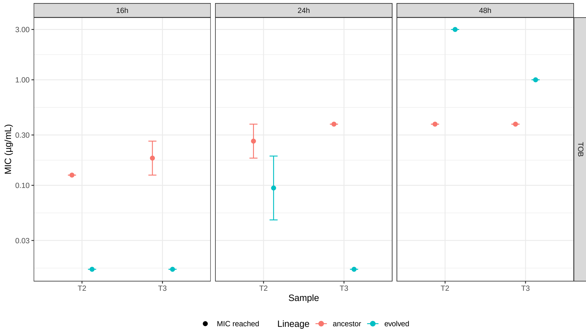
MIC at sampled timepoints (geometric mean \pm SE)
