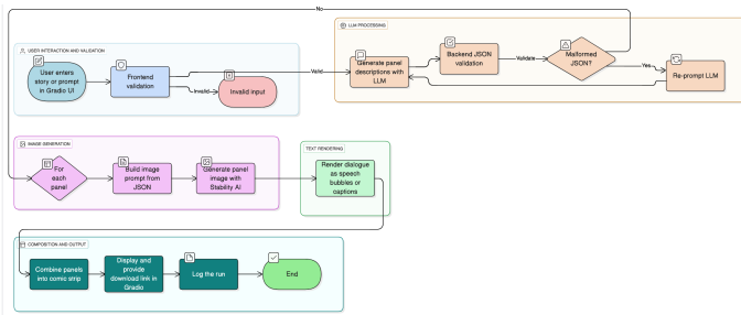
Fig. 1. Workflow
