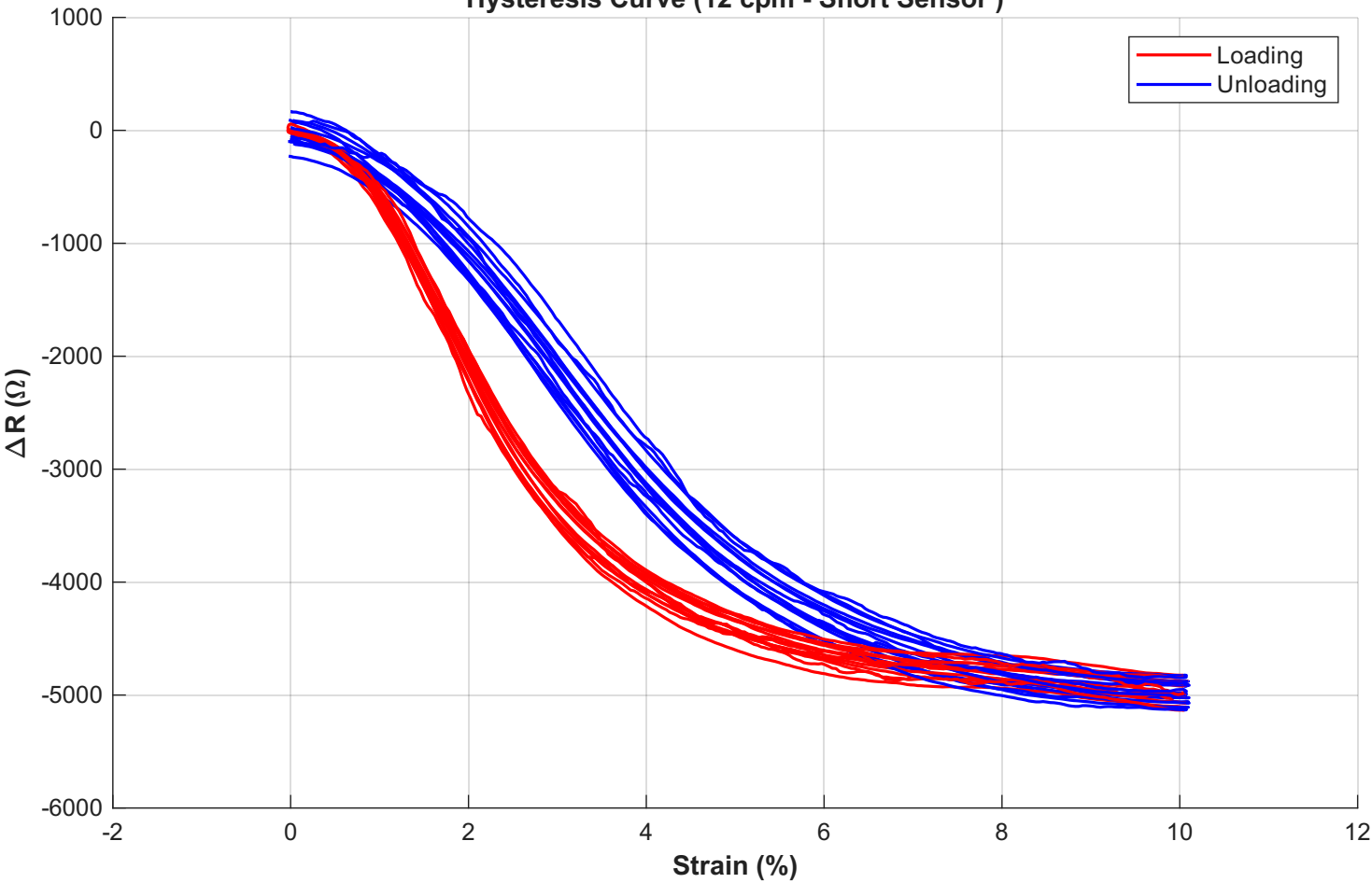
Hysteresis Curve (12 cpm - Short Sensor )
