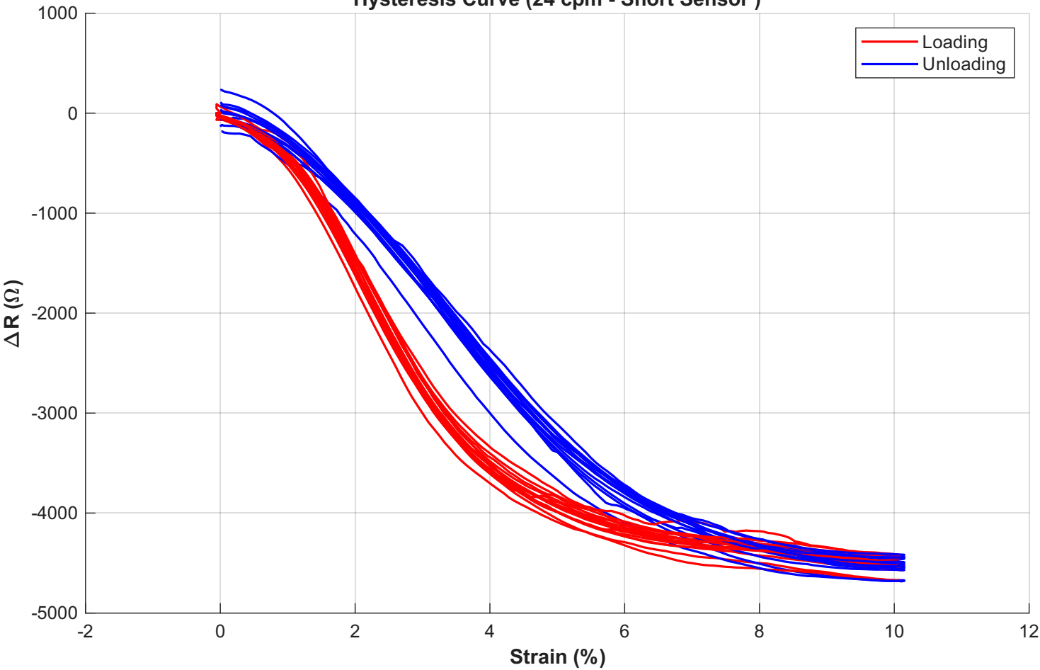
Hysteresis Curve (24 cpm - Short Sensor )
