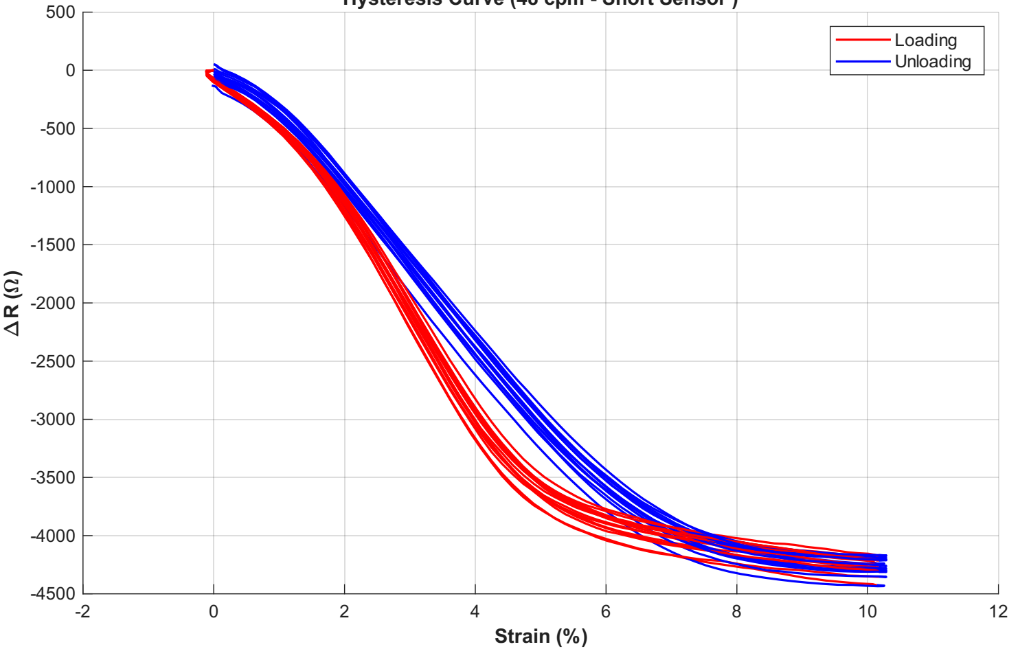
Hysteresis Curve (48 cpm - Short Sensor )
