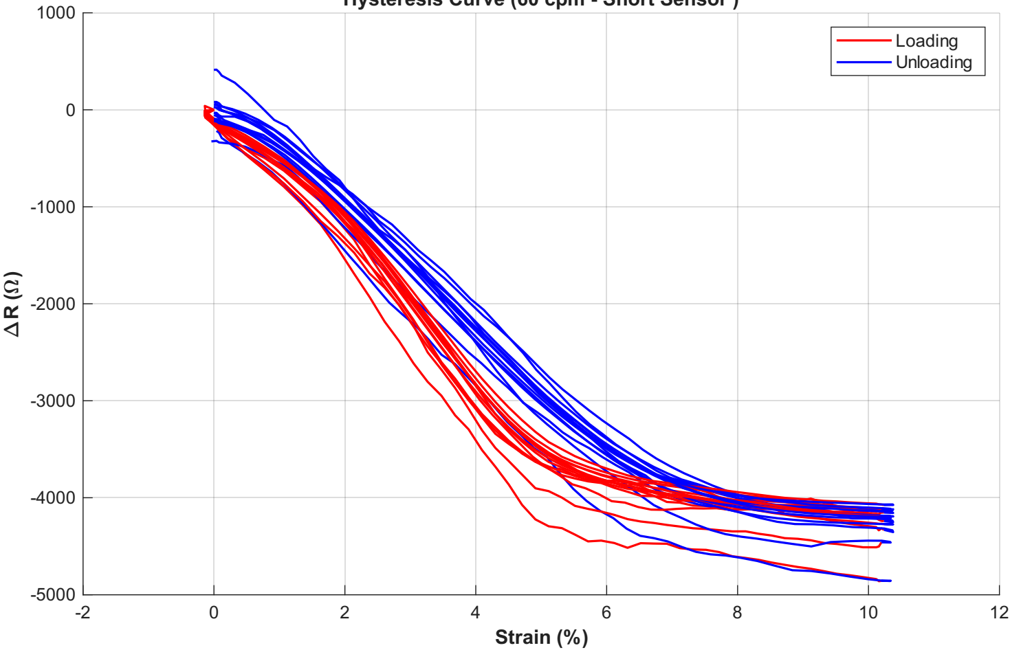
Hysteresis Curve (60 cpm - Short Sensor )
