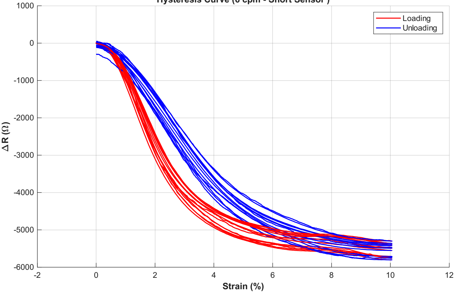
Hysteresis Curve (6 cpm - Short Sensor )
