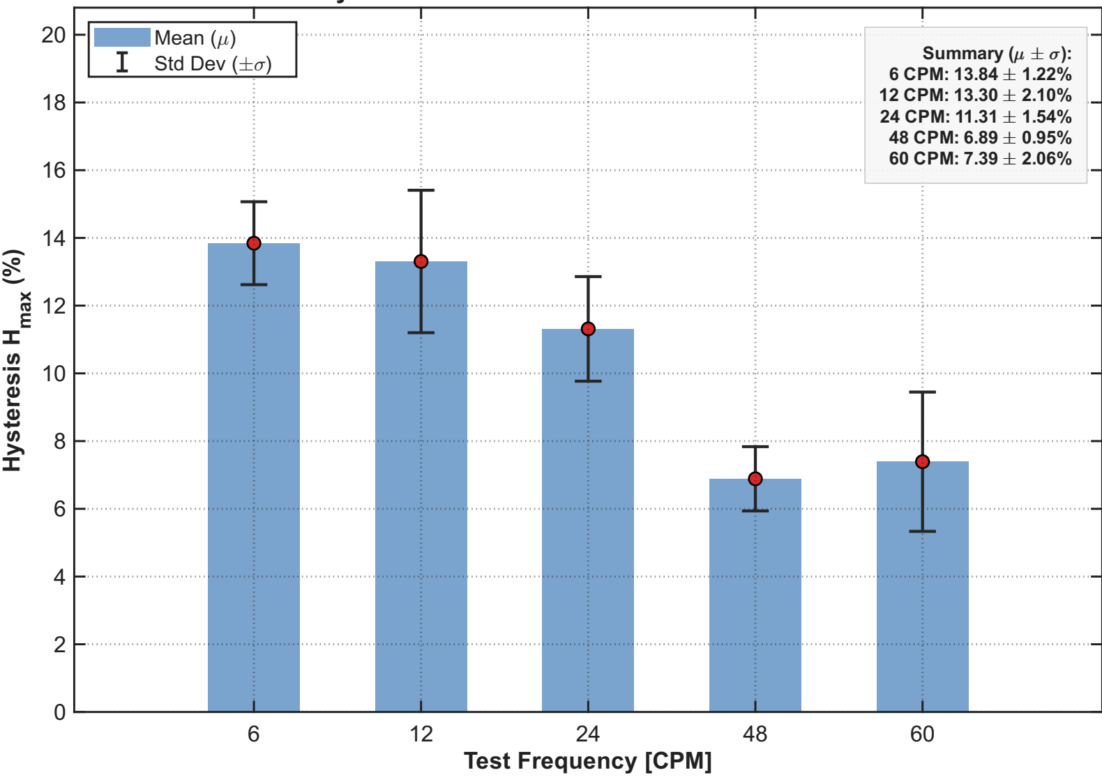
Mean Hysteresis and Standard Deviation - Short Sensor
