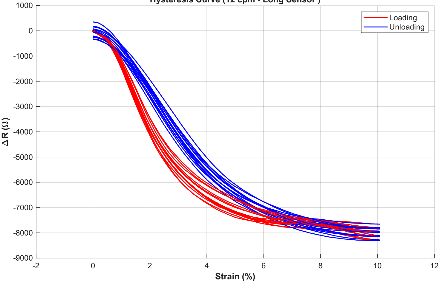
Hysteresis Curve (12 cpm - Long Sensor )
