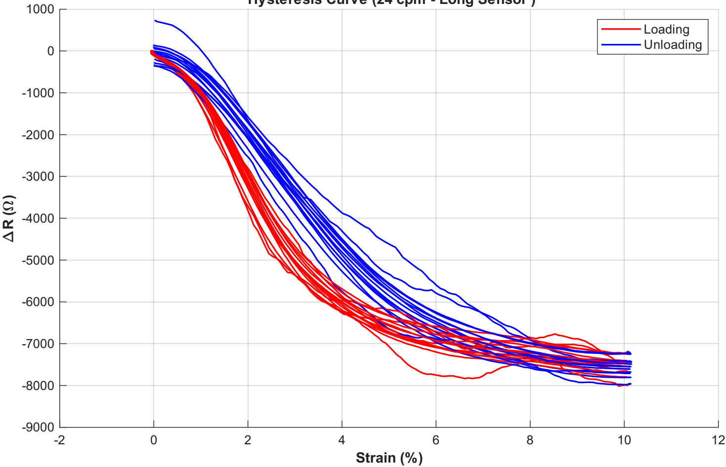
Hysteresis Curve (24 cpm - Long Sensor )
