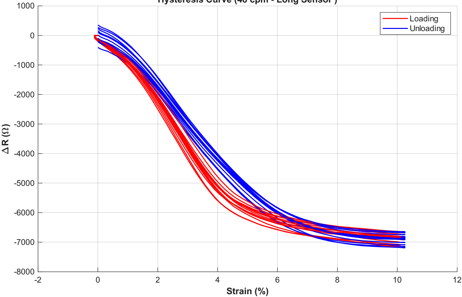
Hysteresis Curve (48 cpm - Long Sensor )
