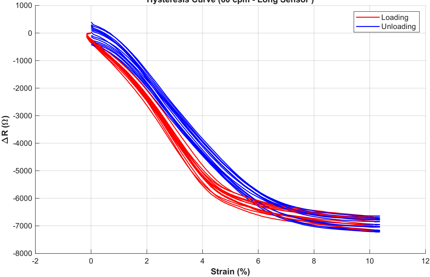
Hysteresis Curve (60 cpm - Long Sensor )
