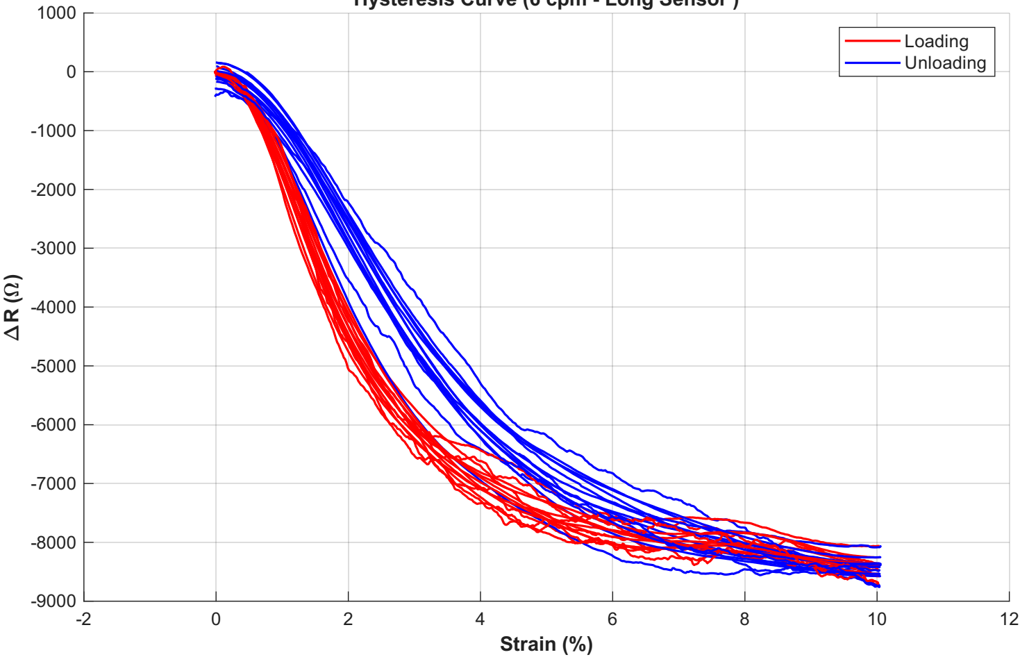
Hysteresis Curve (6 cpm - Long Sensor )
