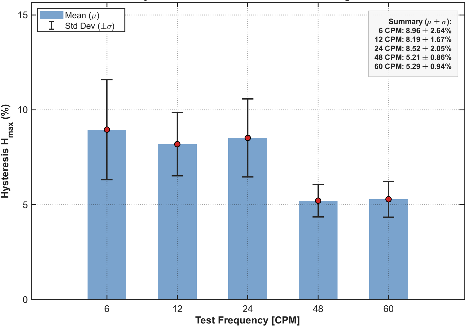
Mean Hysteresis and Standard Deviation - Long Sensor
