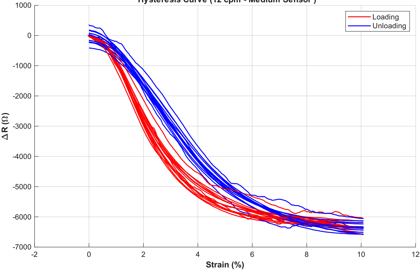
Hysteresis Curve (12 cpm - Medium Sensor )
