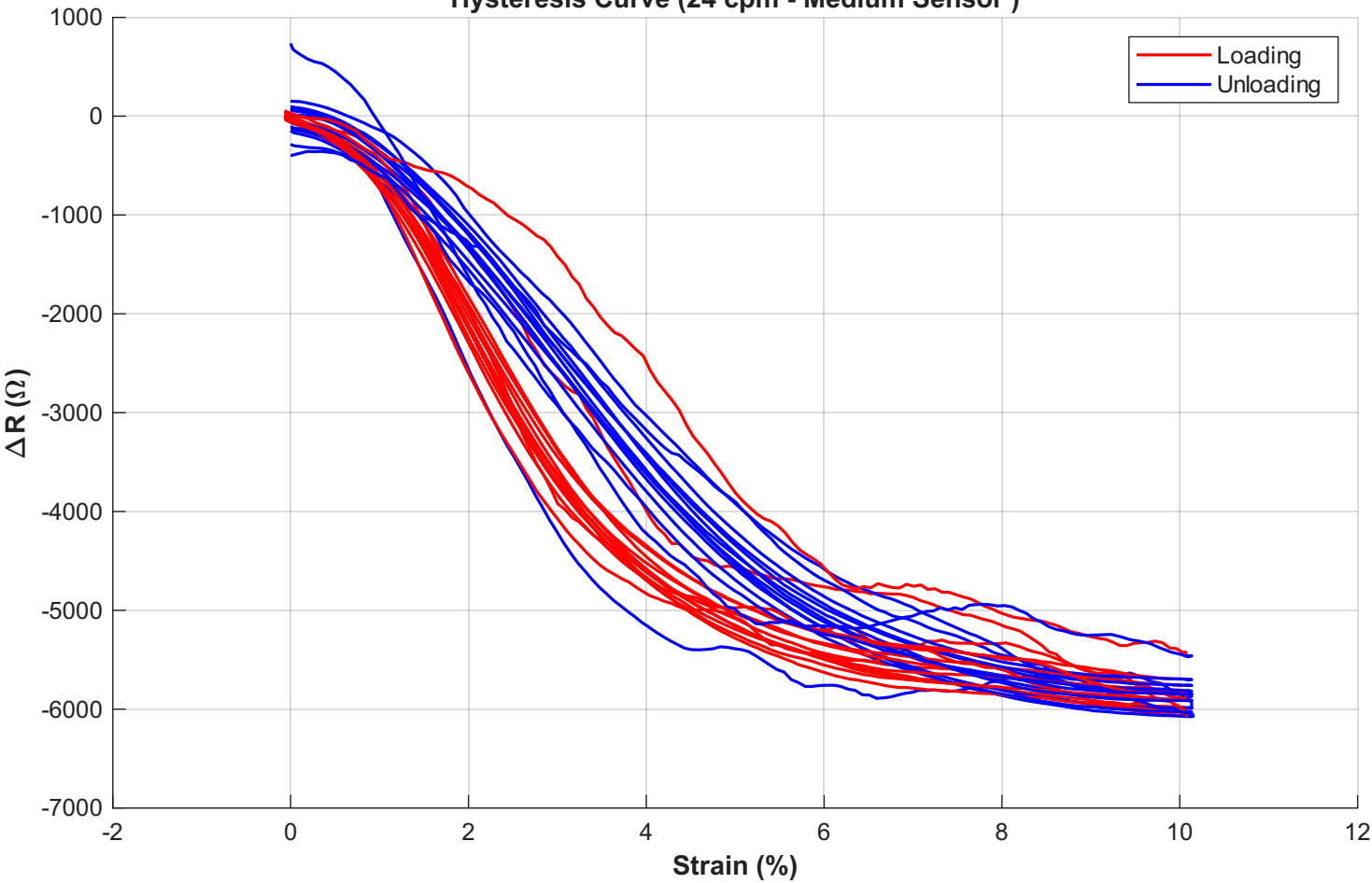
Hysteresis Curve (24 cpm - Medium Sensor )
