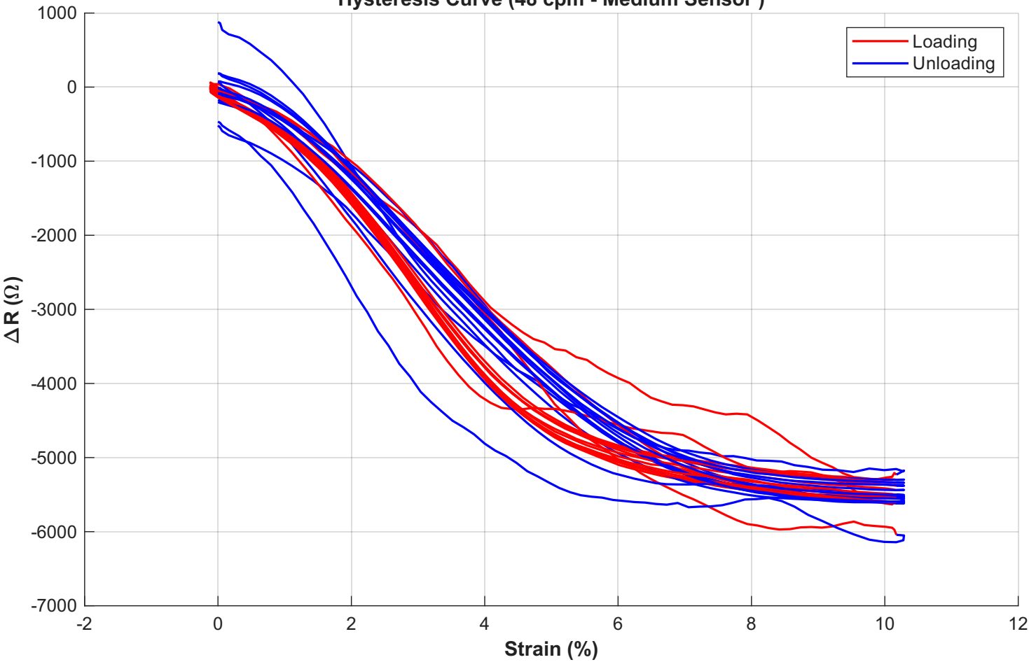
Hysteresis Curve (48 cpm - Medium Sensor )
