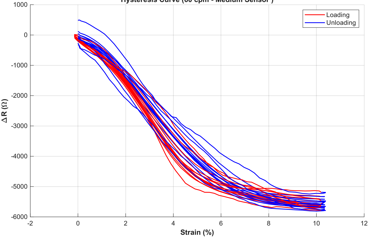
Hysteresis Curve (60 cpm - Medium Sensor )
