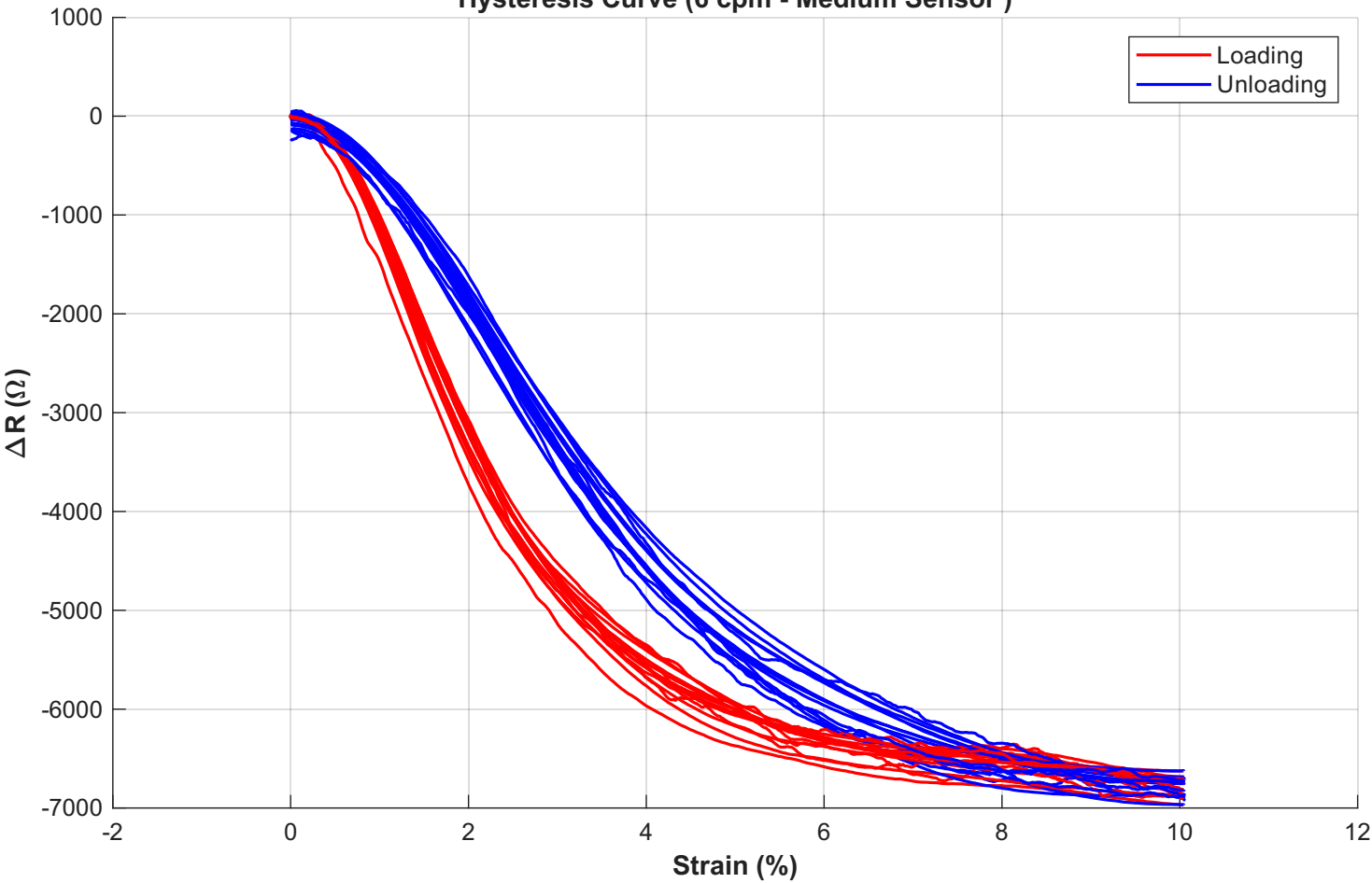
Hysteresis Curve (6 cpm - Medium Sensor )
