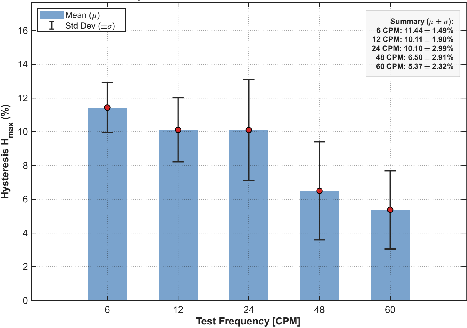
Mean Hysteresis and Standard Deviation - Medium Sensor
