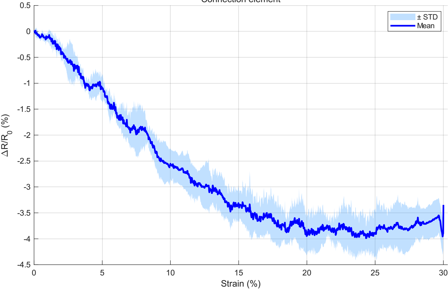
Static response Connection element
