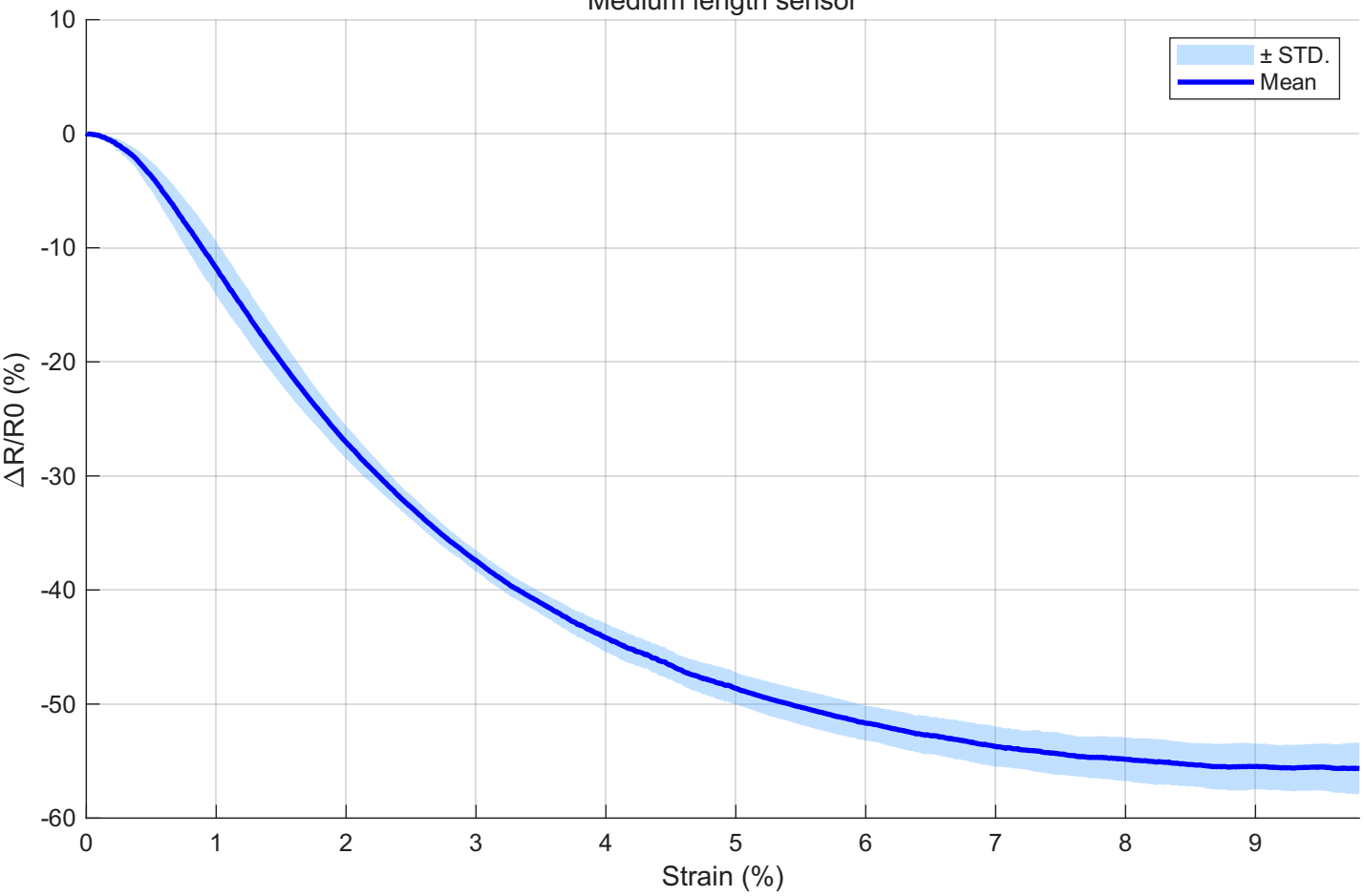
Static response Medium length sensor
