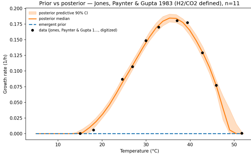
Fig. 2 | Prior (emergent) vs posterior methanogen TPC against Jones 1983.
