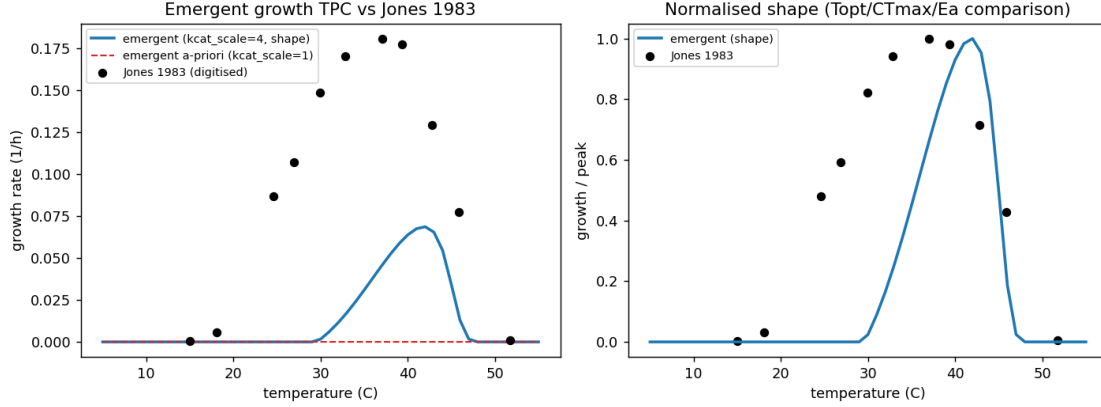
Fig. 1 | Emergent (nothing-fit) methanogen TPC vs Jones 1983: the falling limb (CTmax) matches a-priori; the rising limb and magnitude are calibrated in M4.
