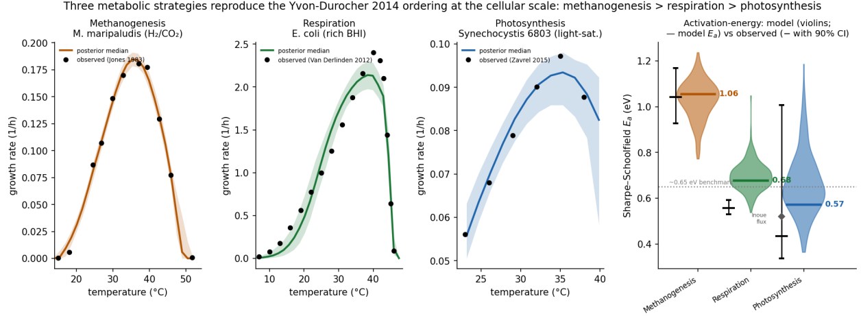
Fig. 1 | Three metabolic strategies reproduce the Yvon-Durocher 2014 activation-energy ordering at the cellular scale. Calibrated (Bayesian) growth thermal performance curves for M. maripaludis methanogenesis ( \text{H}_2/\text{CO}_2 ), E. coli respiration (rich BHI) and Synechocystis 6803 photosynthesis (light-saturated autotrophy): posterior-predictive median and 90% band with the observed data 5–7 . Right: the Sharpe–Schoolfield E_a — violins show the posterior spread, the coloured line and label the model E_a (the decomposition target: 1.06 / 0.68 / 0.57 eV); black markers are the observed E_a with 90% CI (Jones 1.04, Van Der Linden 0.56, Zavrel-growth 0.44 — the phototroph’s wide interval reflects only six rising-limb points, and the model value lies inside it). The grey diamond is the phototroph’s independent Inoue light-saturated flux E_a (0.52), a cross-check, not the observed growth value. The model E_a are correctly ordered, with methanogenesis separated above respiration and photosynthesis near the \sim 0.65 eV benchmark (dotted).
