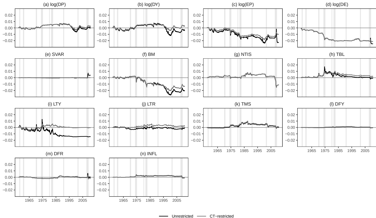
Figure 6.1 Cumulative Differences in Squared Forecast Errors, 1957:01–2010:12
