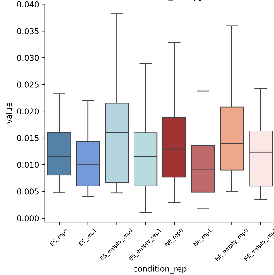
metric = raw_entropy
