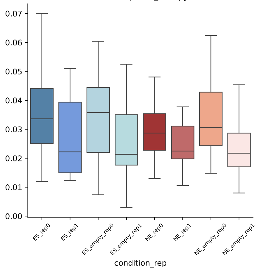
metric = phasic_entropy
