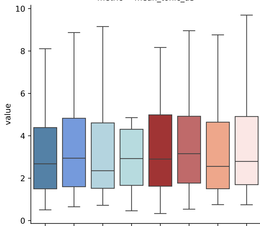
metric = mean_tonic_uS
