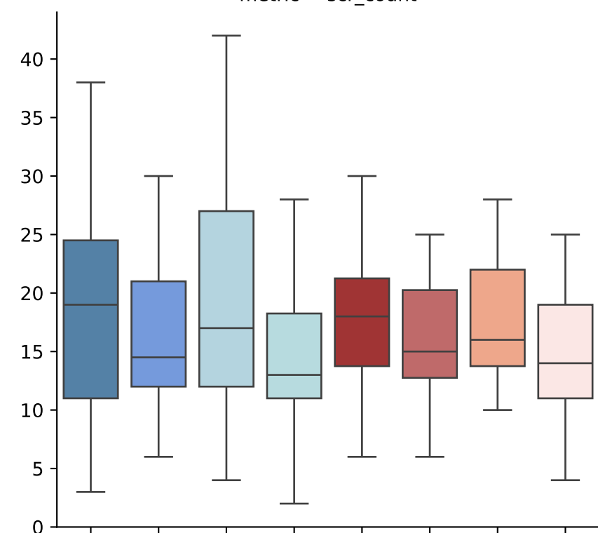
metric = scr_count
