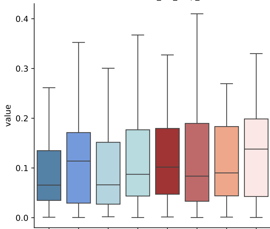
metric = mean_scr_amp_uS
