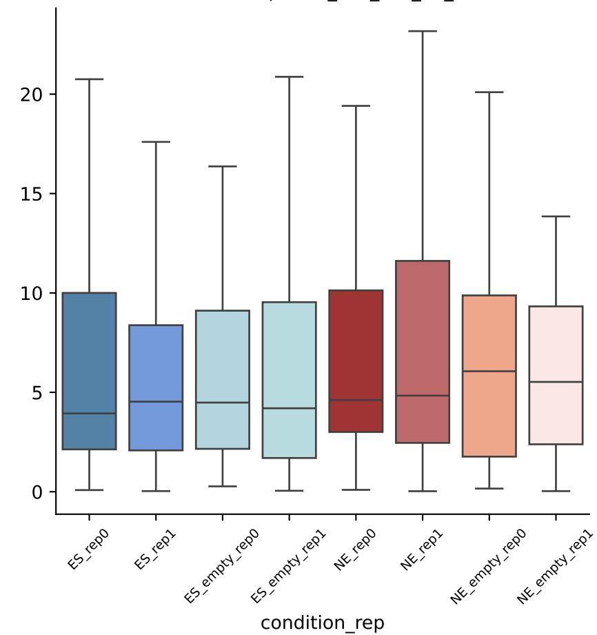
metric = phasic_auc_abs_uS_s
