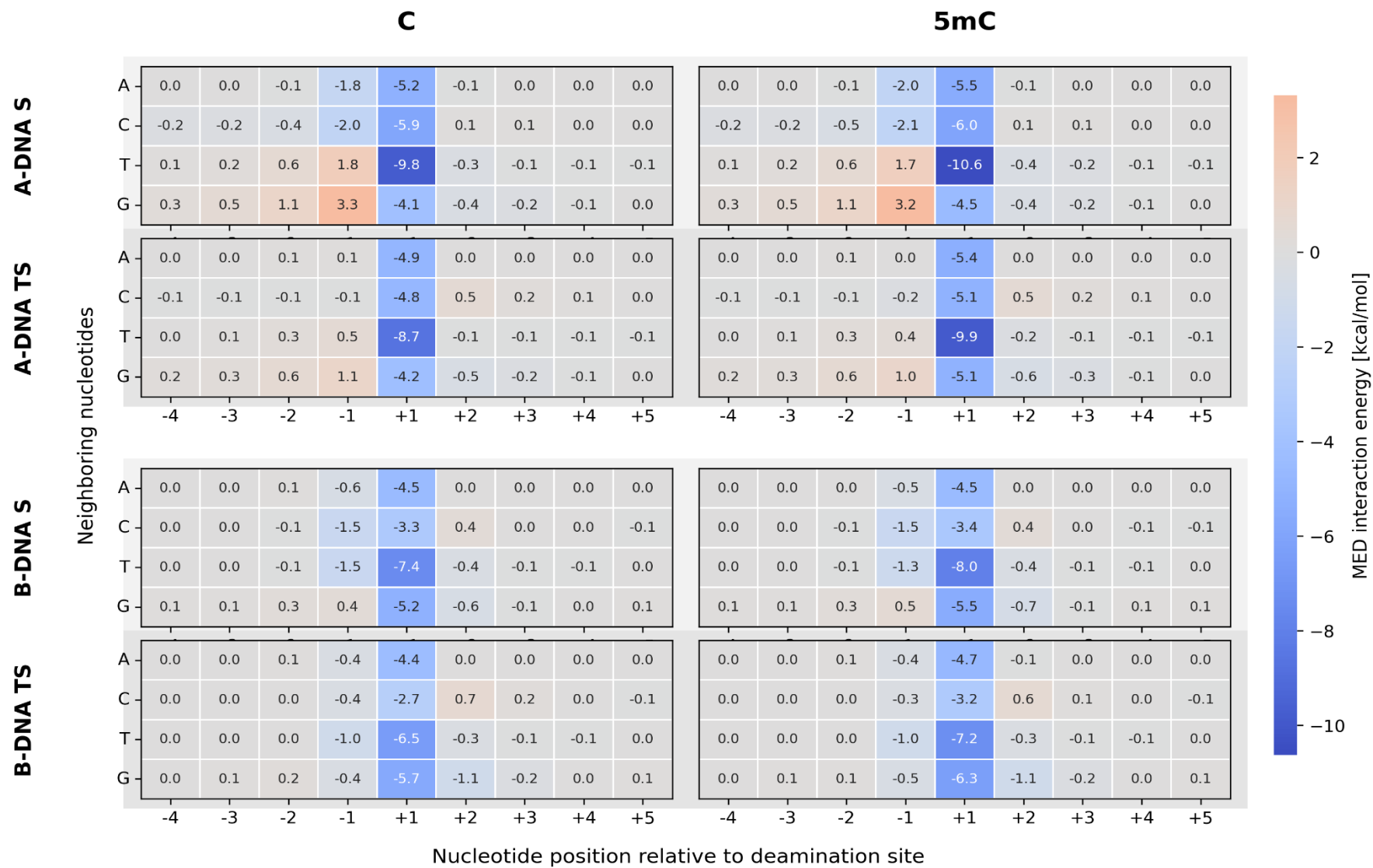
Fig. 5 Heatmaps of MED interaction energies for substrate (S) and transition state (TS) models of C and 5mC deamination in A and B-DNA models.
