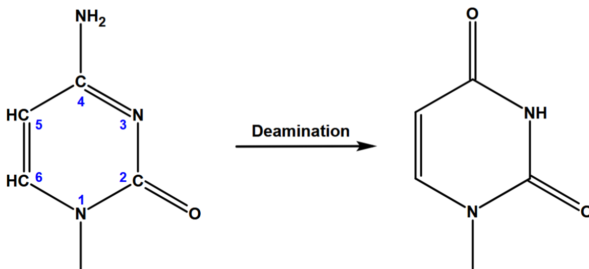
Fig. 1 Deamination of cytosine to uracil.
