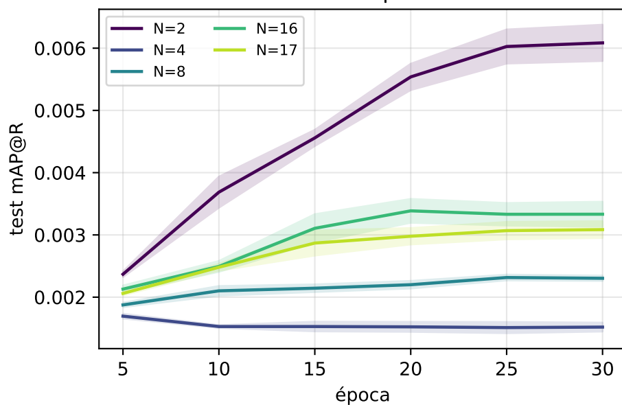
cub200 · profile
