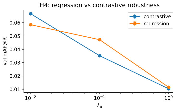
Figure 9: H4: validation mAP@R vs \lambda_g for regression and contrastive. Both peak at small \lambda_g and collapse by \lambda_g=1 ; no clear robustness advantage for contrastive at n=1 .
