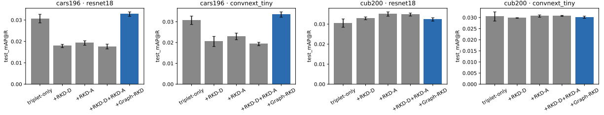
Figure 5: Median test mAP@R per student, one facet per (dataset, teacher) cell (H1). Graph-RKD (blue) is best on both Cars cells; on CUB the classic RKD variants are competitive. CUB is two-seed (provisional).
