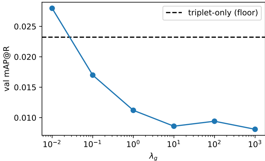
H0: \lambda_g viability gate
