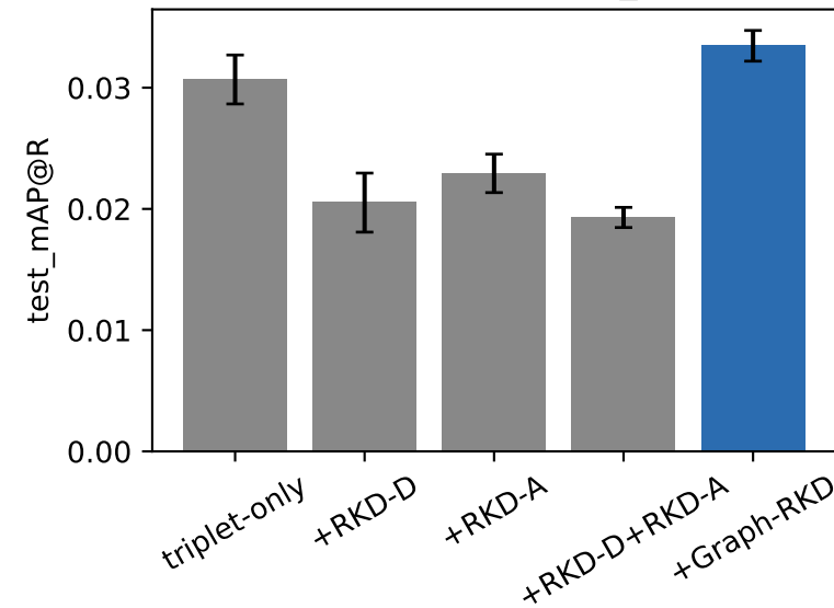
cars196 · convnext_tiny
