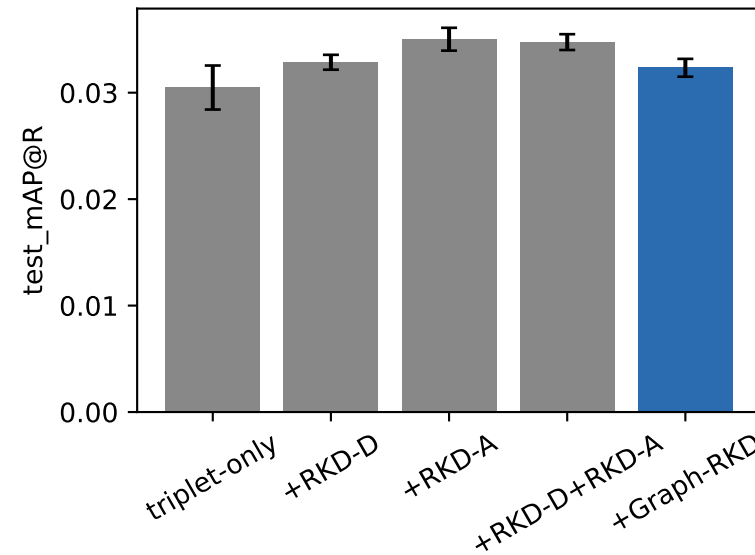
cub200 · resnet18
