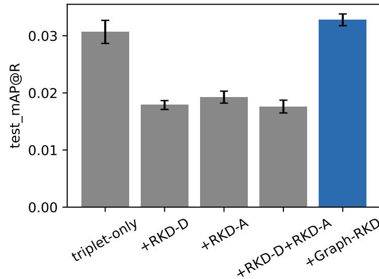
cars196 · resnet18
