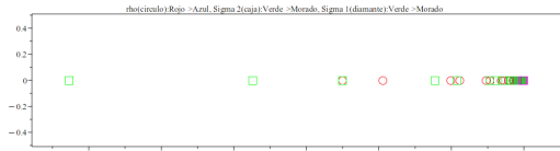
(c) Secuencia de \{\sigma_{1,n}, \sigma_{2,n}, \rho(\mathbf{D}_n)\}_{n=0}^{70} .
