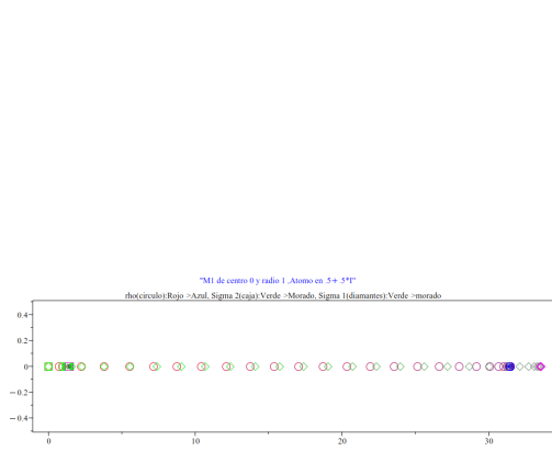
(a) Secuencia de \{\sigma_{1,n}, \sigma_{2,n}, \rho(\mathbf{D}_n)\}_{n=0}^{50} .
