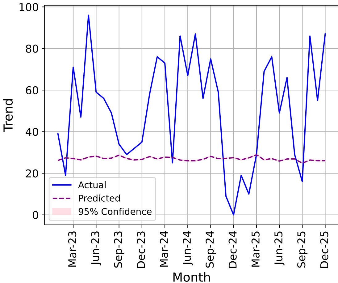
Cluster_4_score
