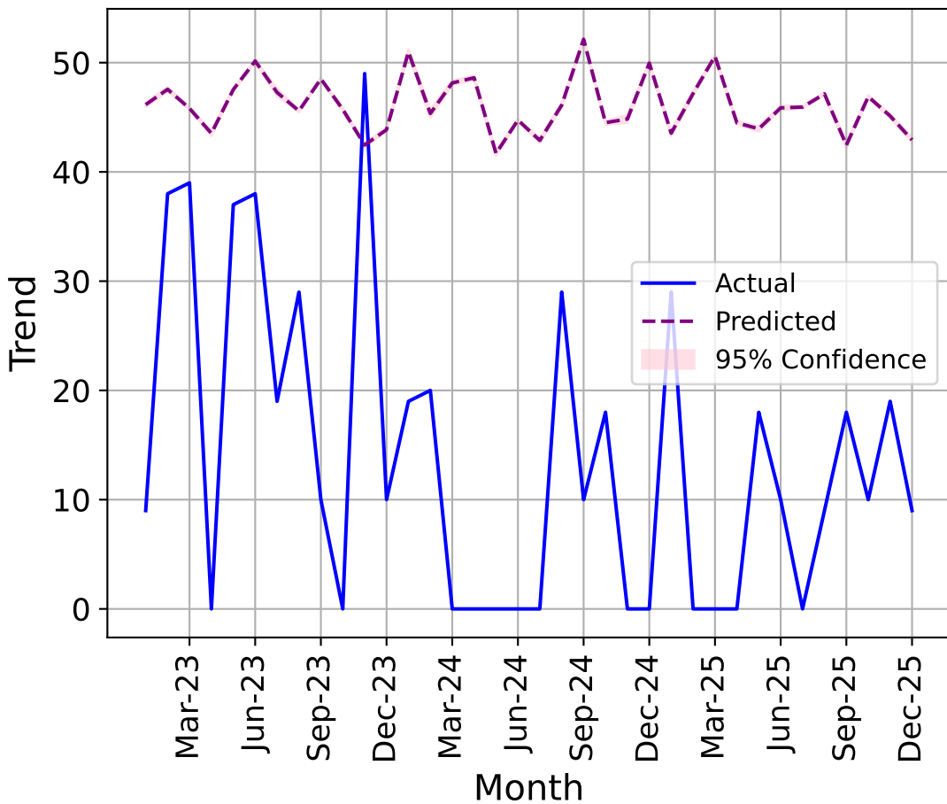
Cluster_5_score
