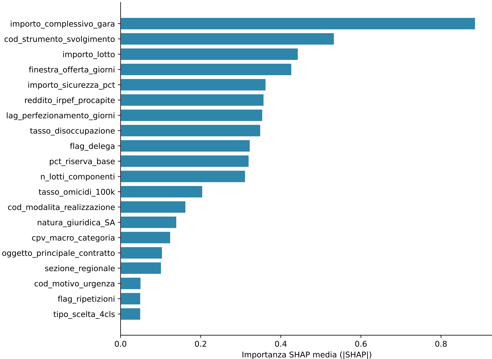
SHAP importanza globale — lgb_supervised M1 Top 20 feature (score grezzo pre-Platt)
