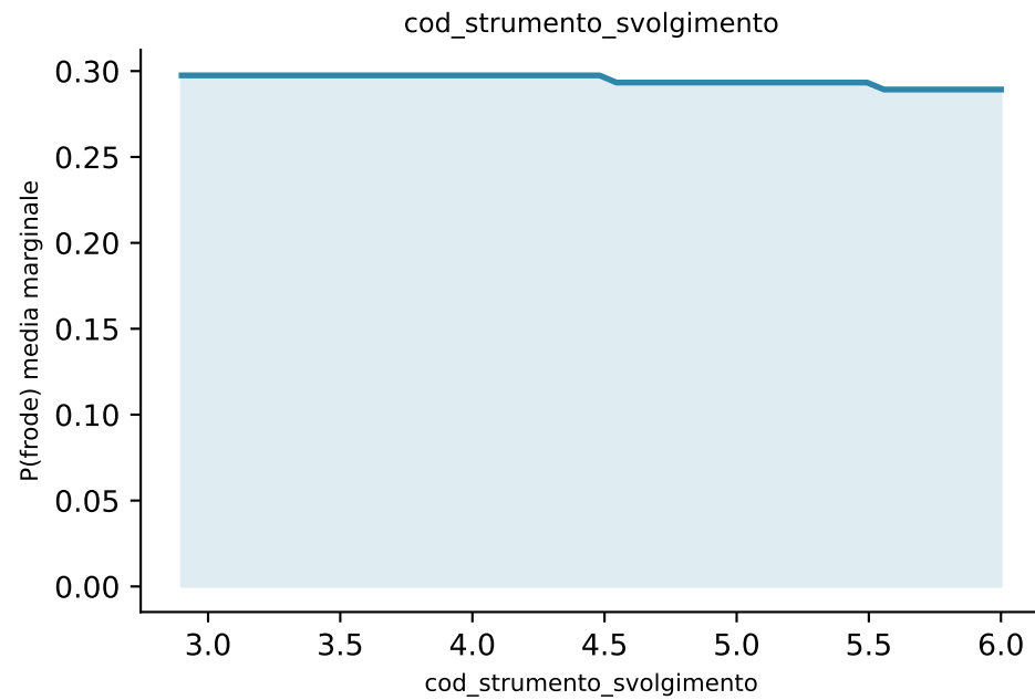
PDP top-3 feature — lgb_supervised M1 (media marginale, score grezzo pre-Platt)
