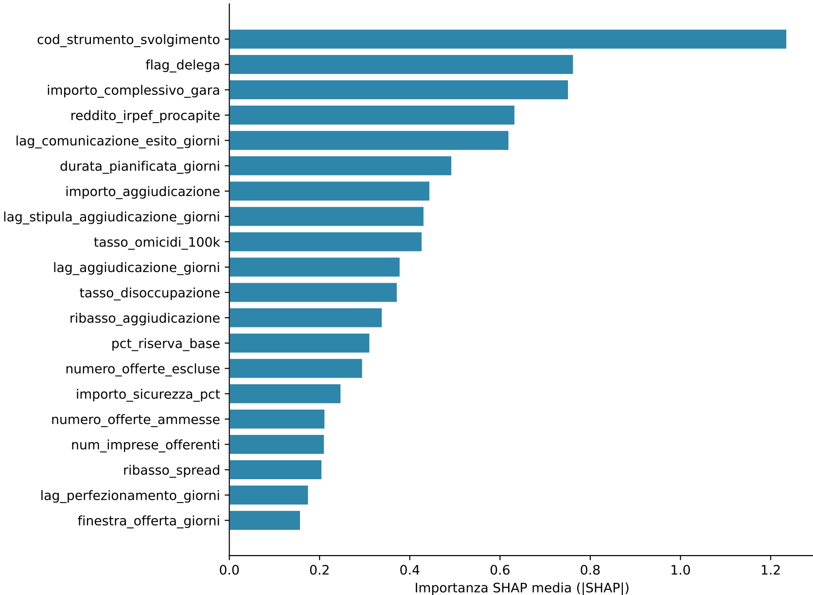
SHAP importanza globale — lgb_supervised M3 Top 20 feature (score grezzo pre-Platt)
