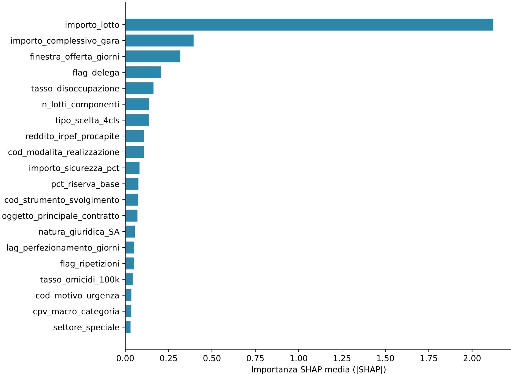
SHAP importanza globale — bagging_lgbm M1 Top 20 feature (score grezzo pre-Platt)
