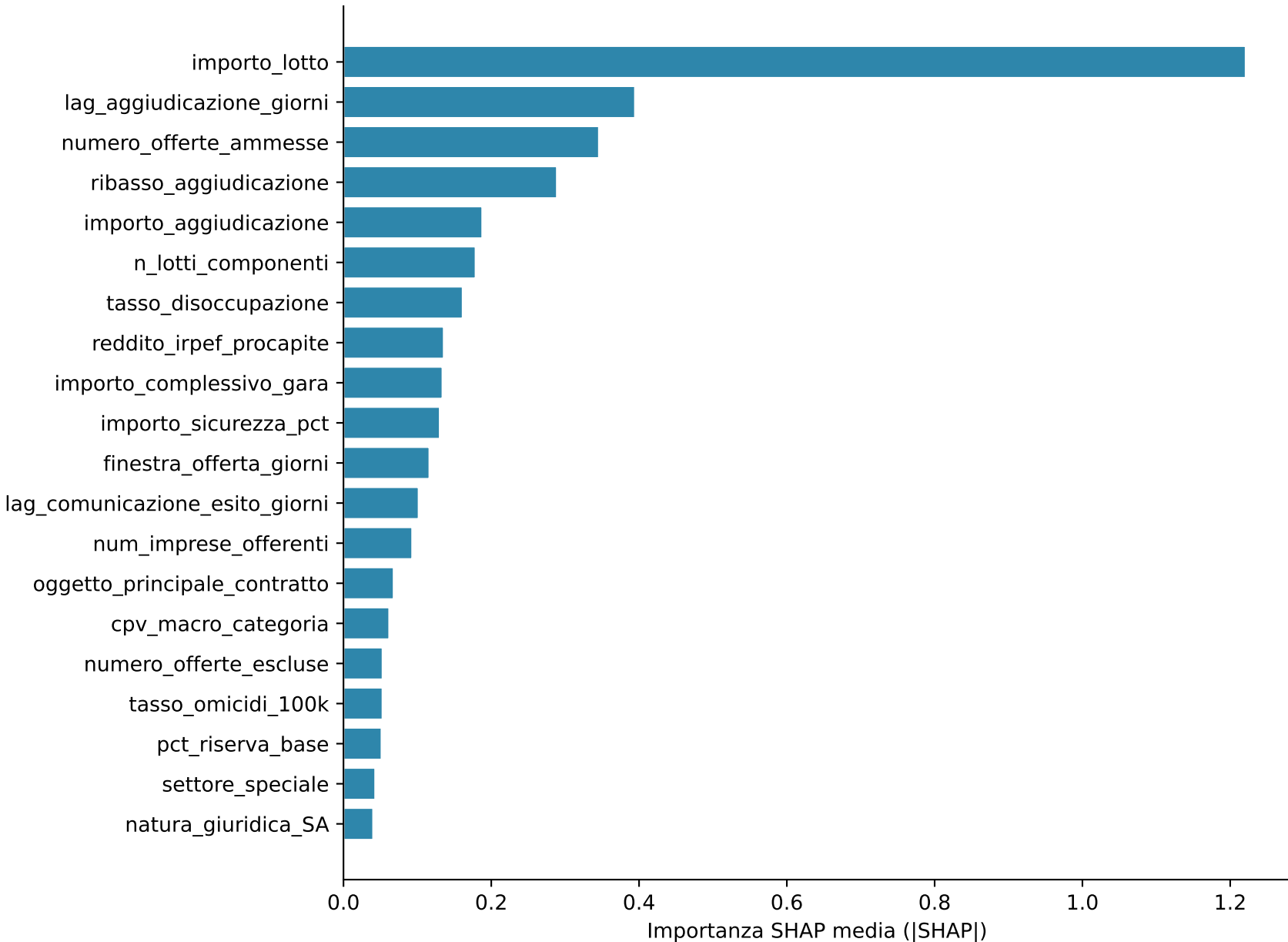
SHAP importanza globale — bagging_lgbm M2 Top 20 feature (score grezzo pre-Platt)
