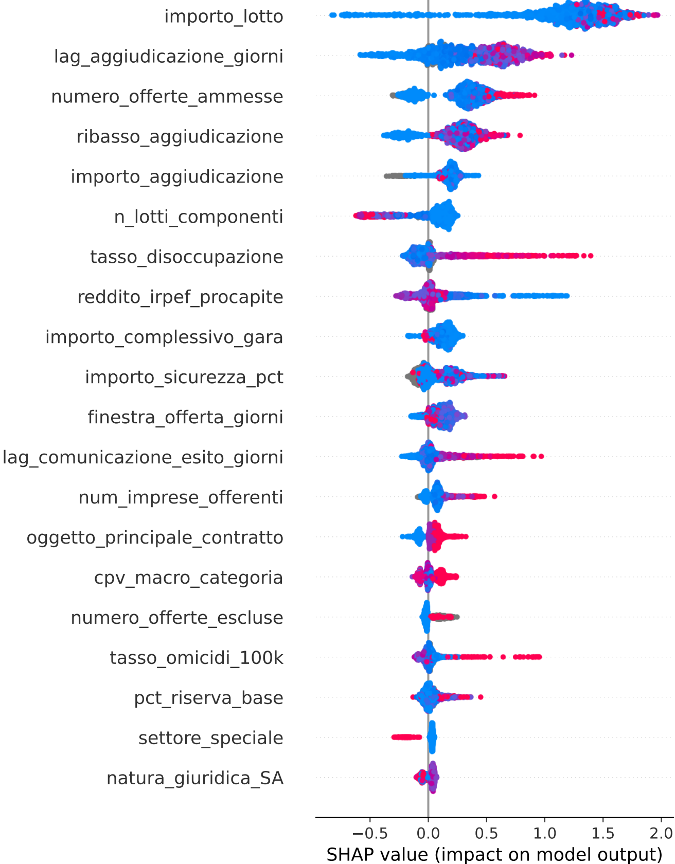
SHAP beeswarm — bagging_lgbm M2 (top 20, score grezzo)
