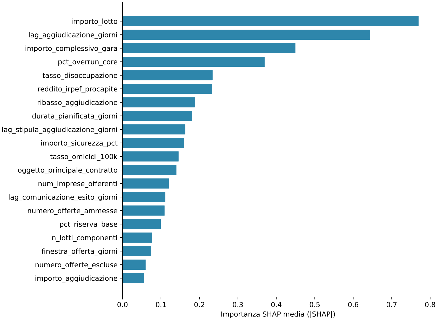
SHAP importanza globale — bagging_lgbm M3 Top 20 feature (score grezzo pre-Platt)
