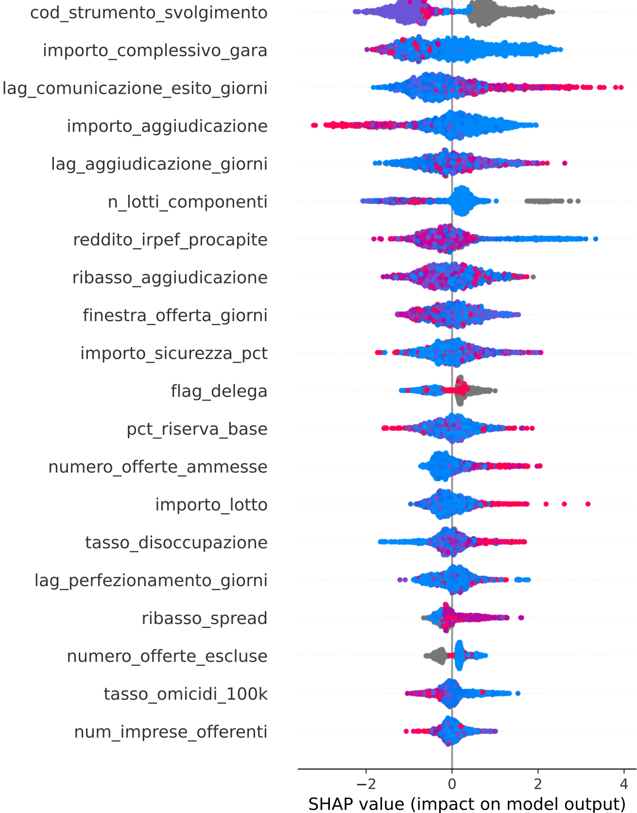
SHAP beeswarm — lgb_supervised M2 (top 20, score grezzo)
