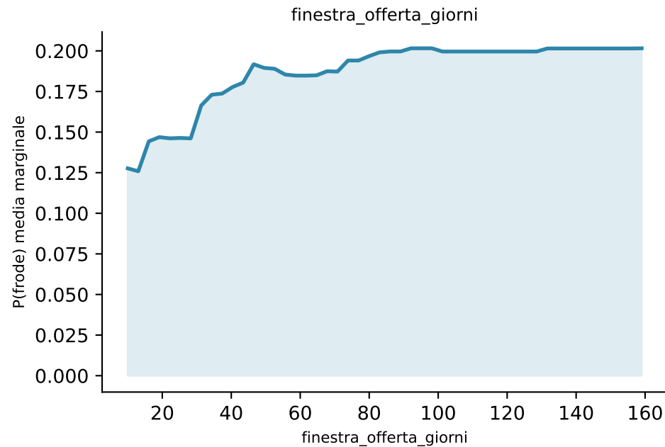
PDP top-3 feature — re_lgbm M1 (media marginale, score grezzo pre-Platt)
