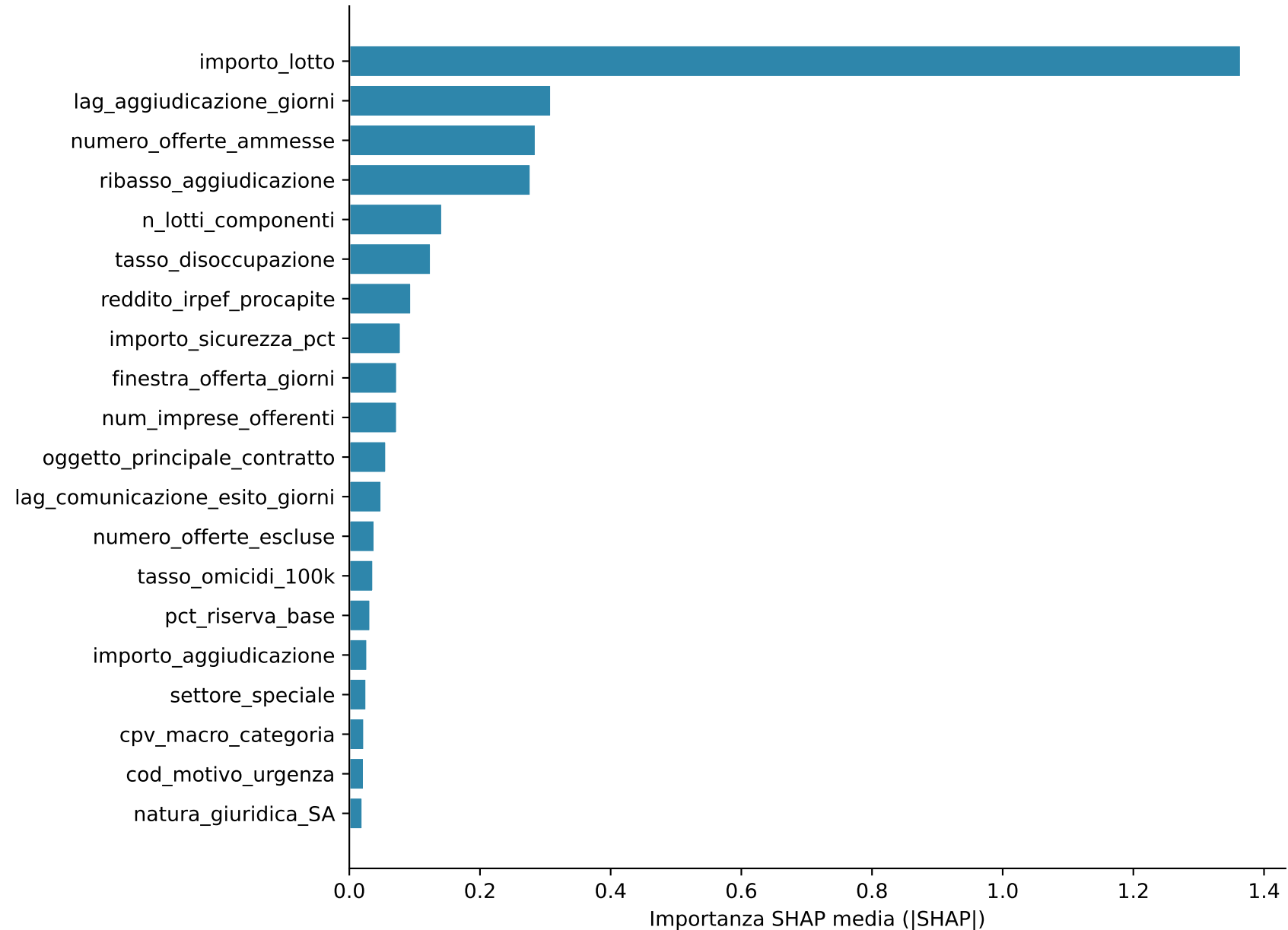
SHAP importanza globale — re_lgbm M2 Top 20 feature (score grezzo pre-Platt)
